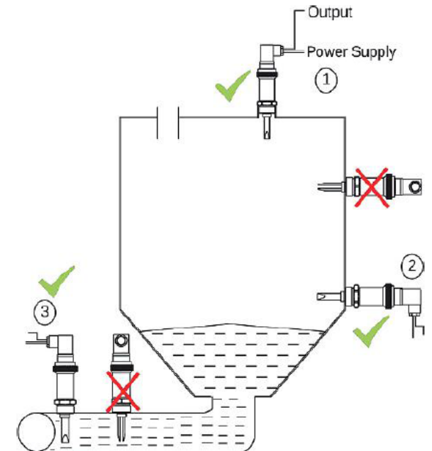
Figure 3: Installation Diagram
