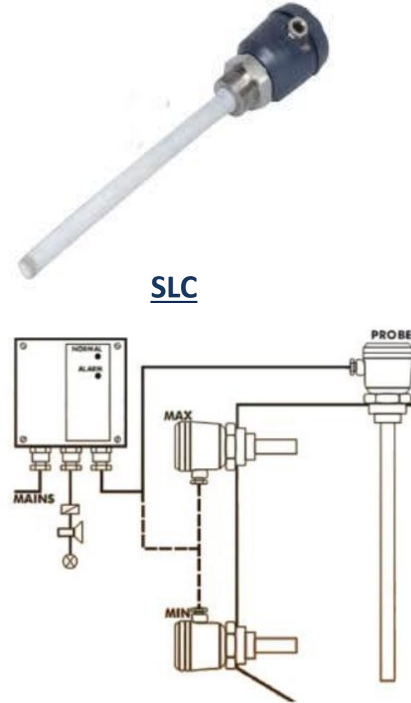
Figure 2: System Diagram
