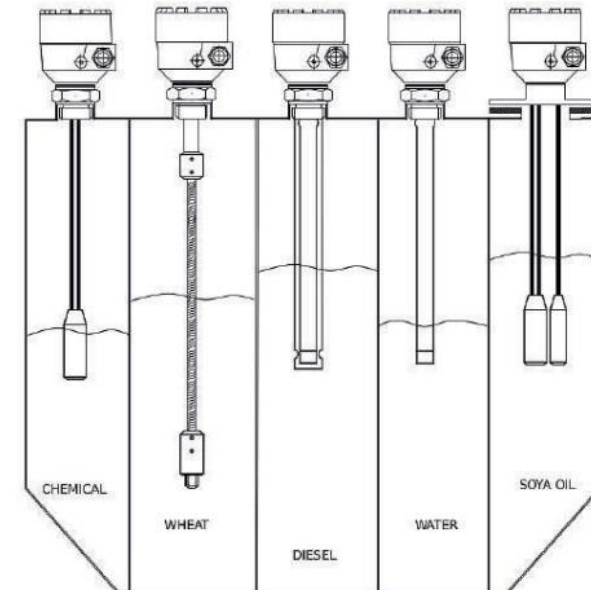
Figure 3: Installation of Various Probes
