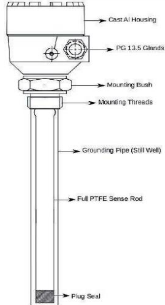
Figure 1: Parts of Capvel ICT
