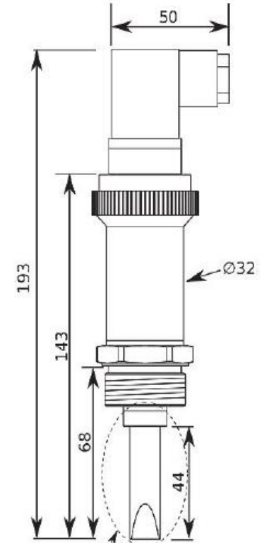
• GA Drawing
